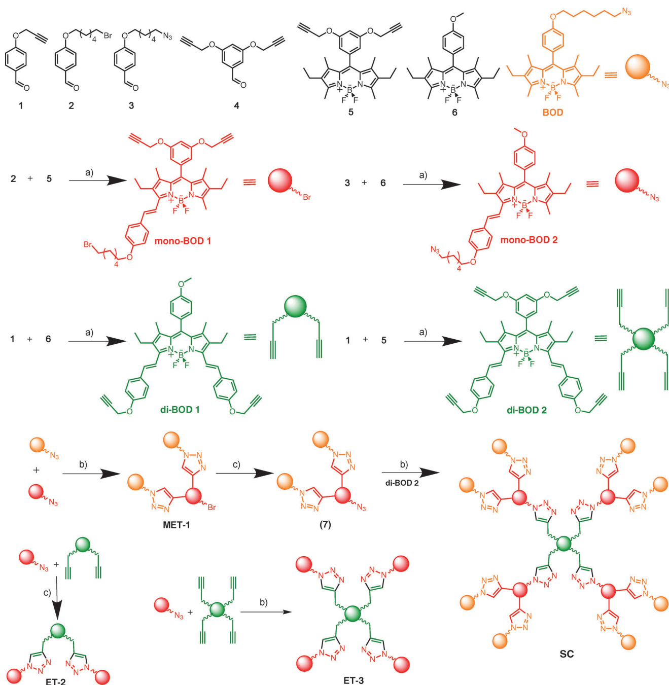
Scheme 1. Synthesis and schematic representations of ET molecules and SC. a) piperidine, AcOH, benzene, reflux; b) \text{CuSO}_4 \cdot 5\text{H}_2\text{O} , \text{Et}_3\text{N} , Sodium Ascorbate, \text{THF:H}_2\text{O} ; c) \text{NaN}_3 , B18C6, acetonitrile, 60^\circ\text{C} . Synthetic procedures for each aldehyde, compounds 5, 6, and all other reaction details and explicit structures can be found in the Supporting Information.
